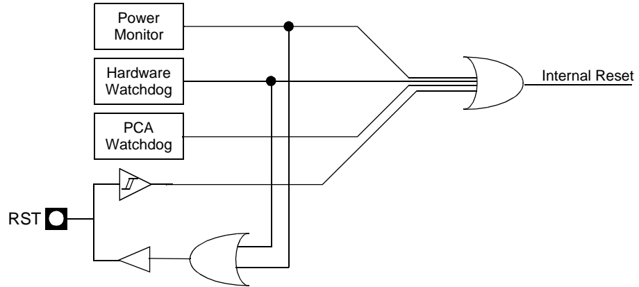
Figure 68. Reset schematic
